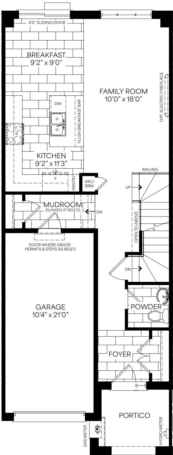
Main Floor Elevation A
